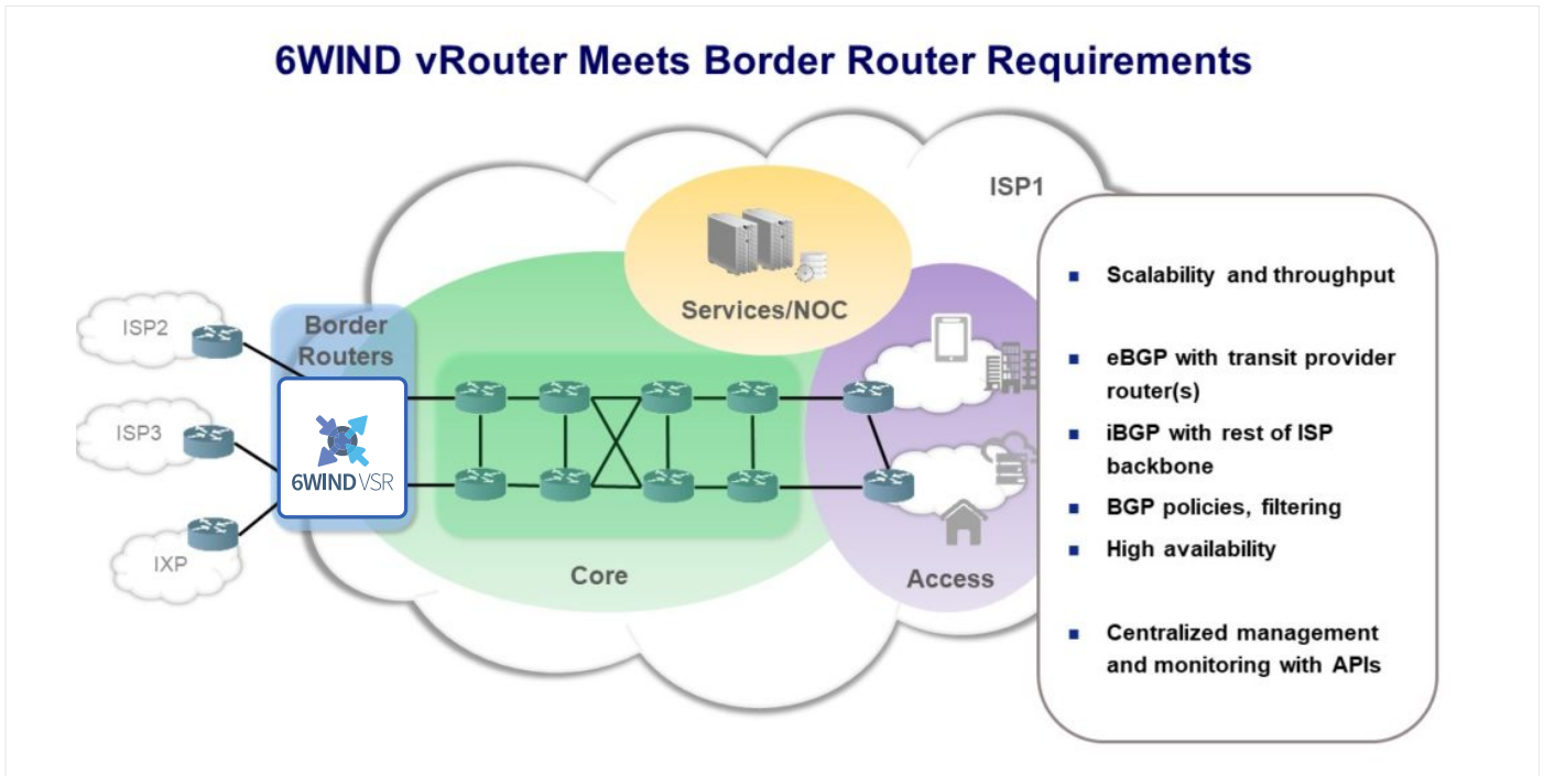
Figure 2. 6WIND border vRouter connects multiple ISP networks. 2
